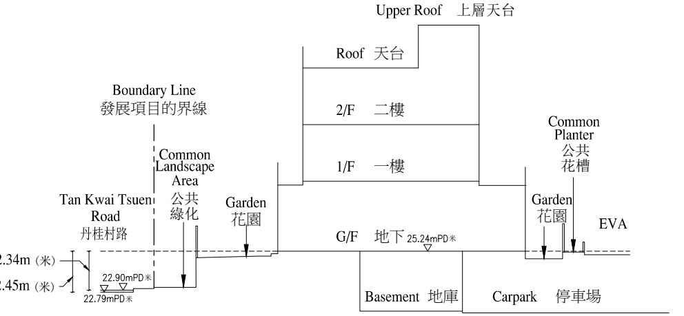
Cross-section Plan (15) 橫截面圖 (15)
