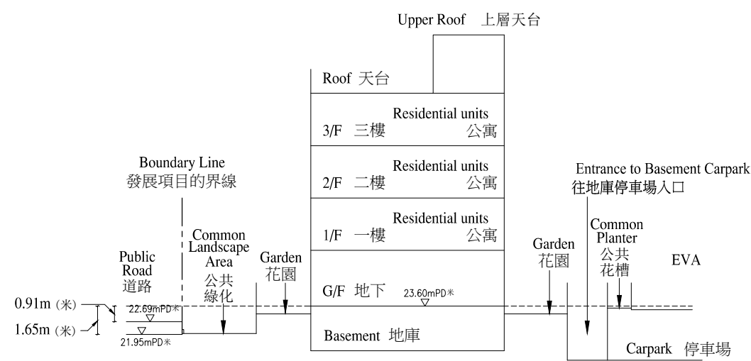
Cross-section Plan (3) 橫截面圖 (3)
