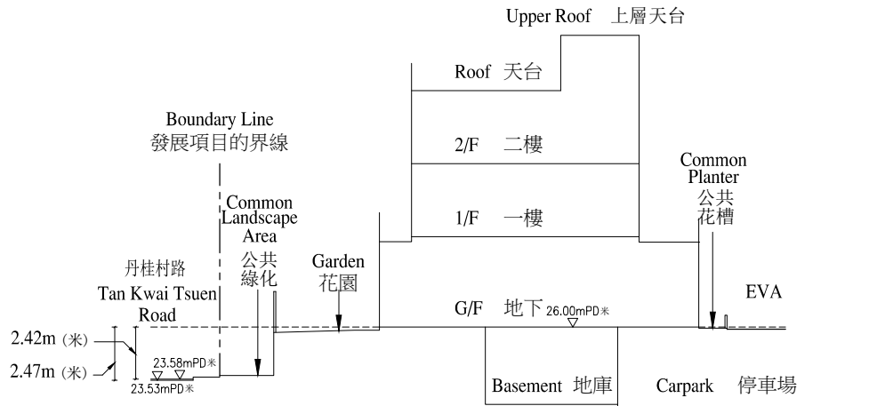
Cross-section Plan (7) 橫截面圖 (7)
